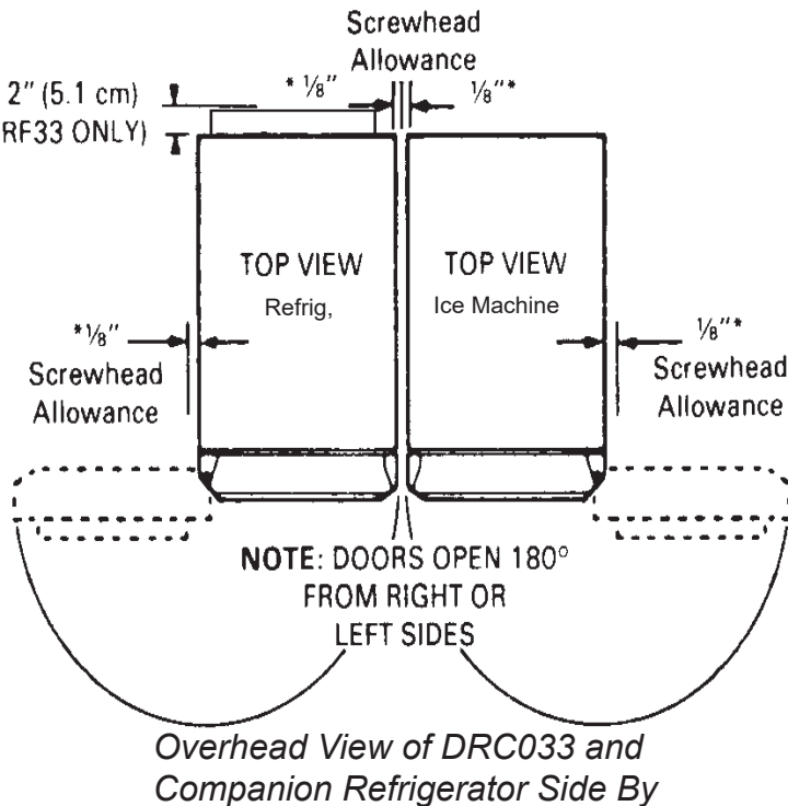
DRC033 Cabinet Views
