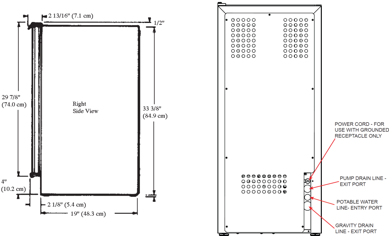
DRC033 Cabinet Views
